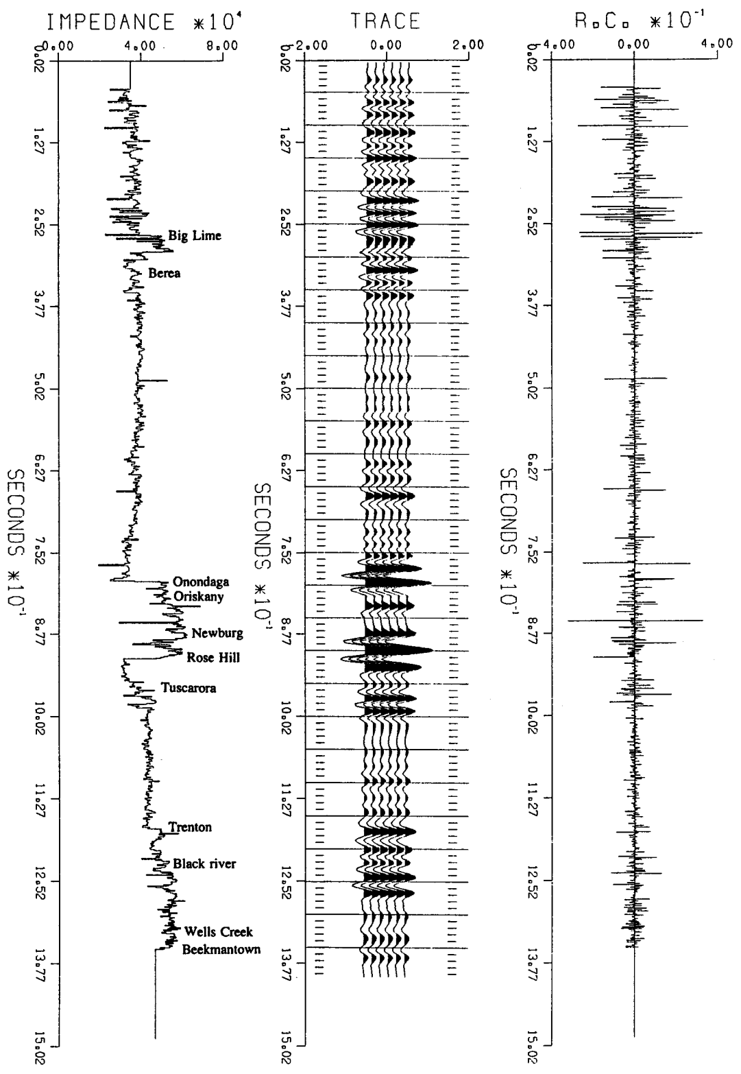
Fig.3.3A Synthetic seismogram for deep well K3462 in Kanawha County
