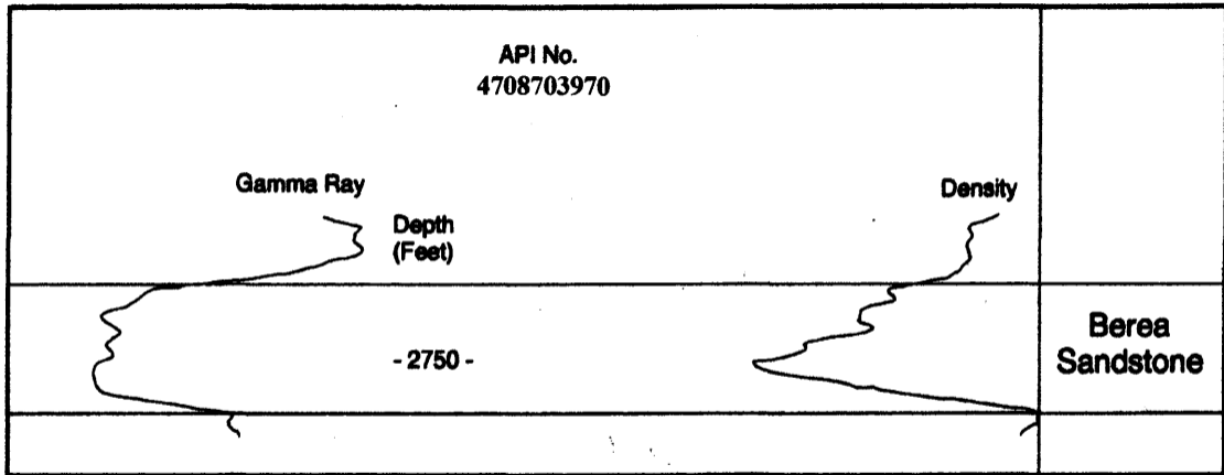
Figure MDe-21. Type geophysical log (API No. 4708703970) for the Berea Sandstone in the Gay-Fink Consolidated field in Doddridge, Lewis, Ritchie, Jackson, and Roane counties, West Virginia. This log is a typical example of the fluvial-deltaic facies in this field.
