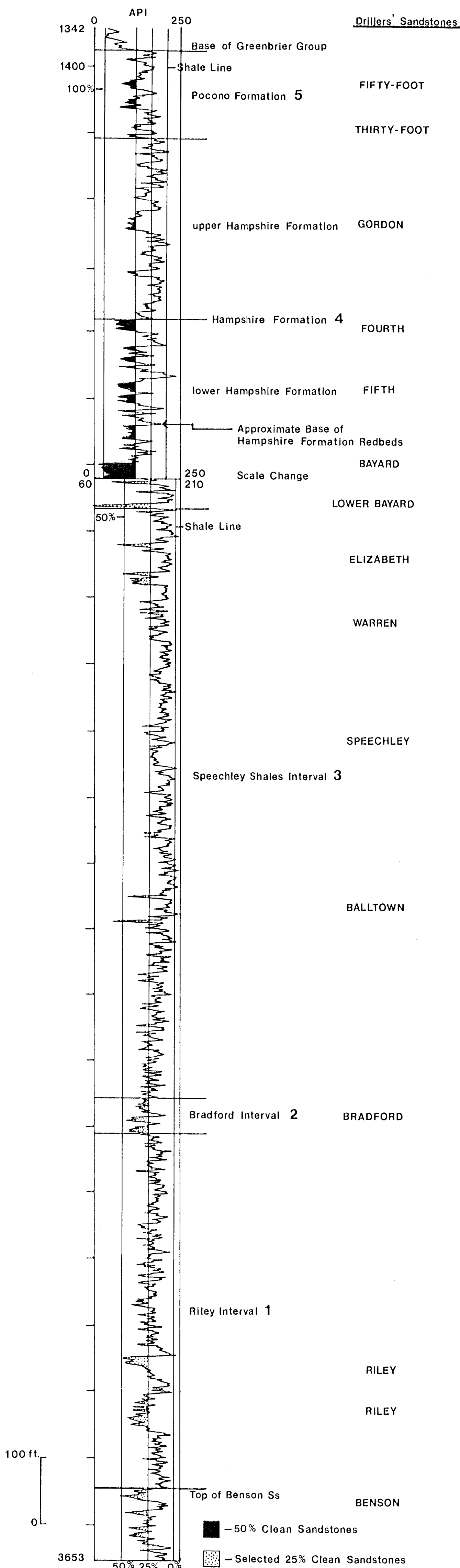
PLATE 2: Major subsurface lithostratigraphic intervals.
