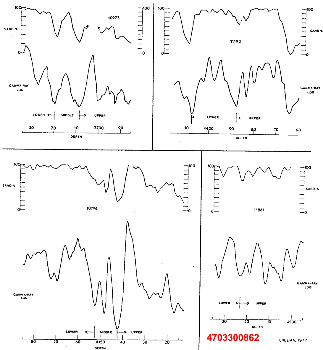
FIG. 4 PLOT SHOWING CLOSE CORRESPONDENCE BETWEEN GAMMA-RAY LOG AND SAND PERCENT IN THE BENSON CORES
