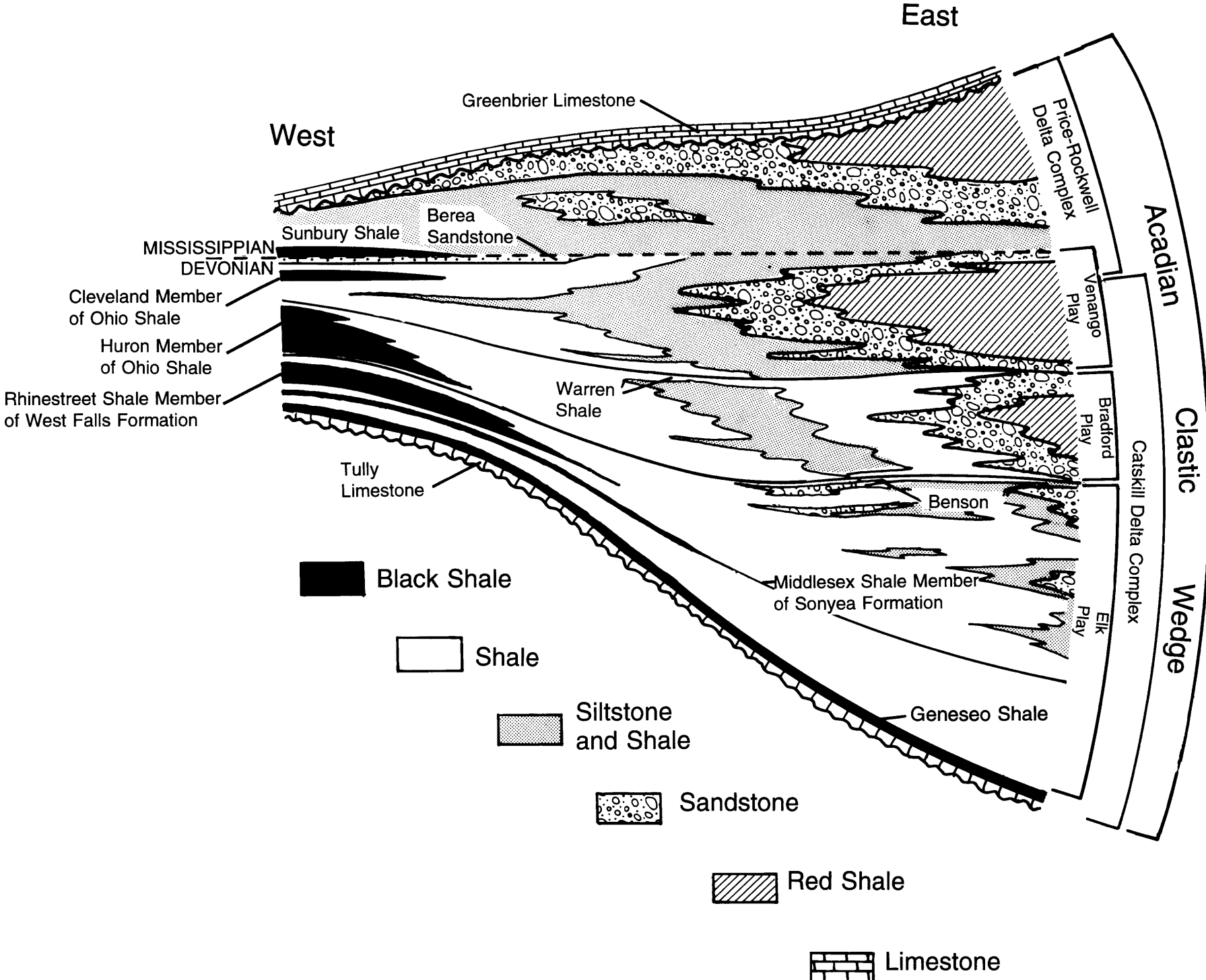
Figure Dvs-3. Diagrammatic cross section of the Acadian clastic wedge, showing the relationship of the Price-Rockwell and Catskill delta complexes, the three sandstone and siltstone plays with key bounding units noted, and the general lithologic framework.
