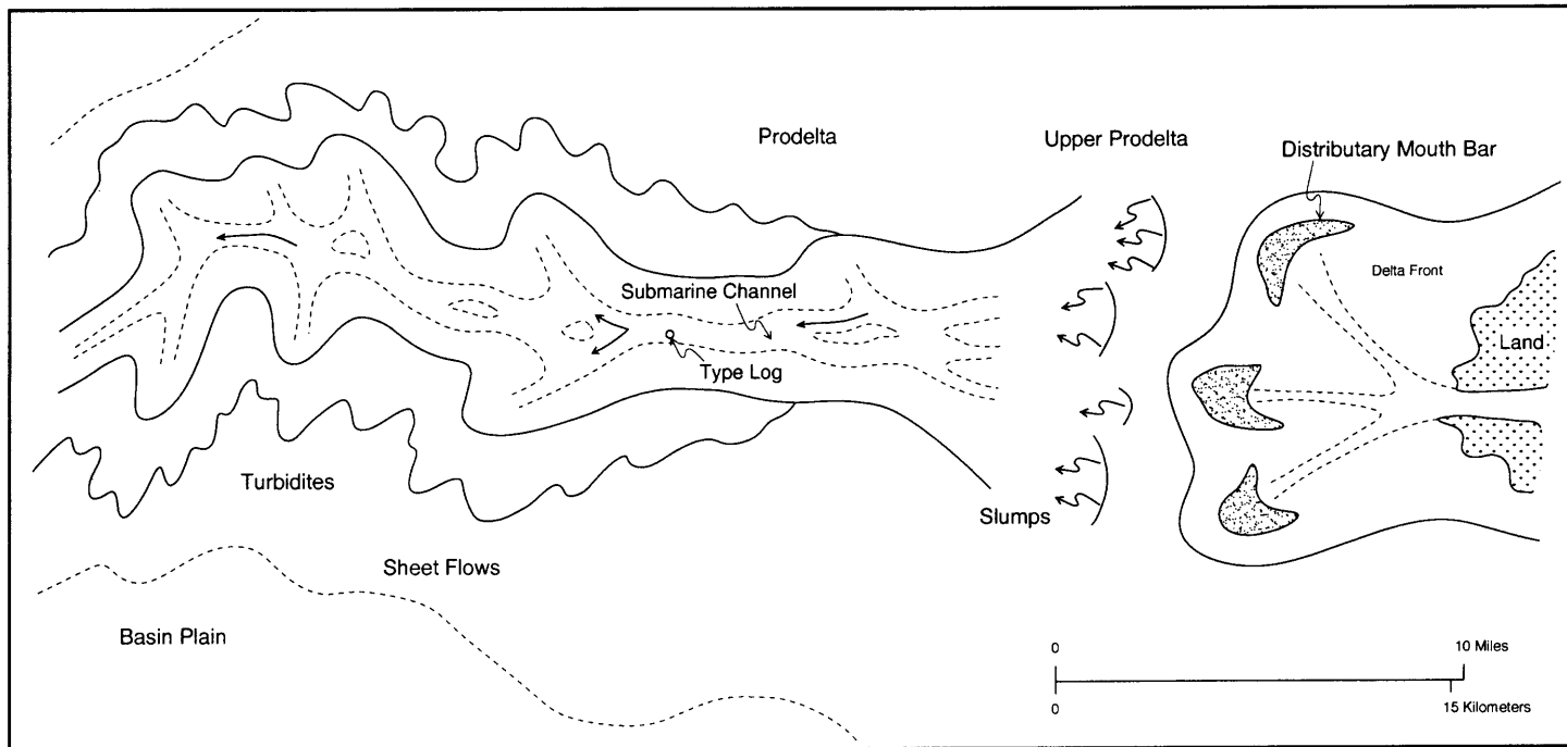
Figure Dvs-26. Paleoenvironments of the Bayard sandstone, northern West Virginia. Location of the type log (Figure Dvs-27) is indicated. Deposition is interpreted to have occurred within a submarine channel fed by periodic upper prodelta slumps associated with a major fluvial-deltaic sediment input system located to the east. From Heim (1987).
