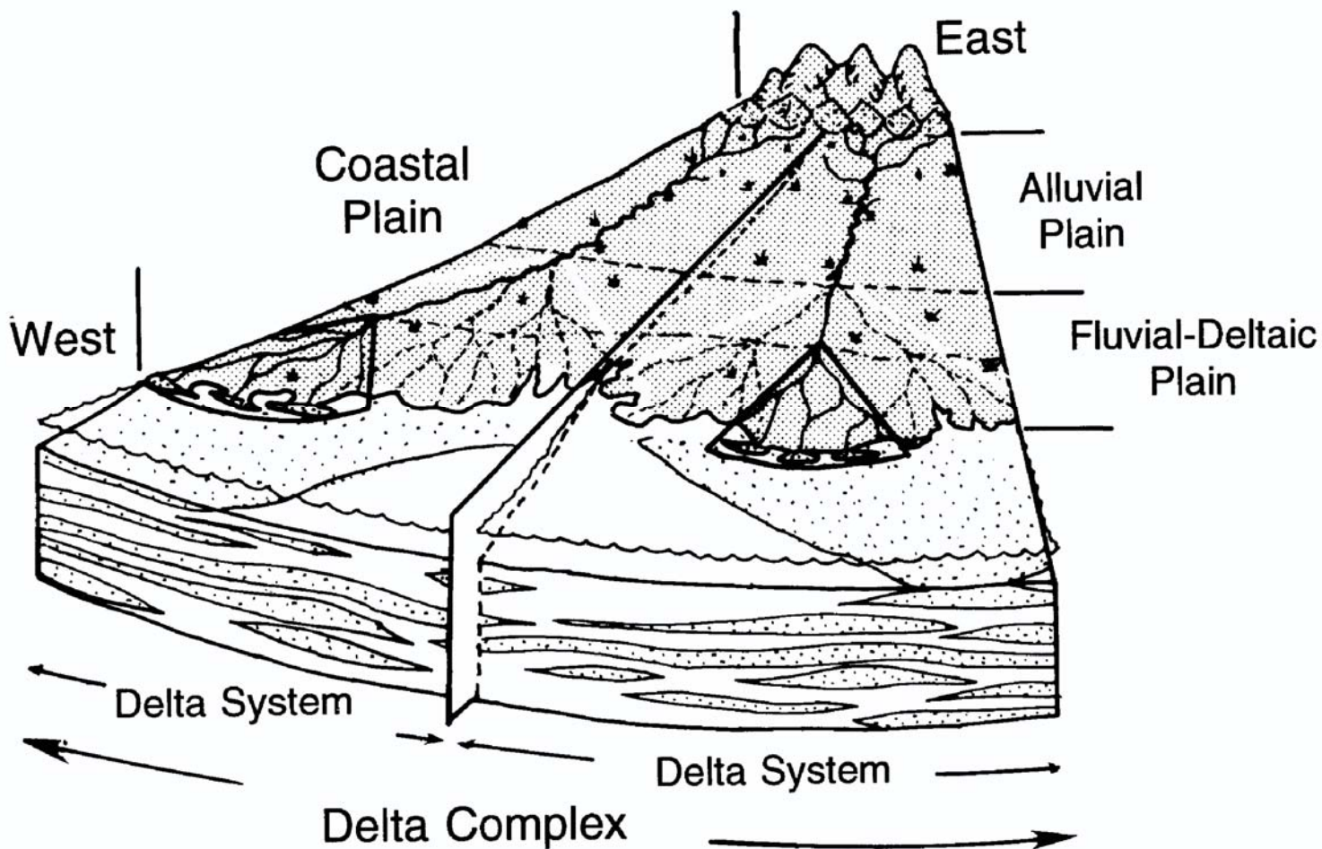
Figure Dvs-12a. Schematic diagram of interpreted Catskill delta complex depositional environments showing the multi-river architecture (Boswell and Donaldson, 1988).
