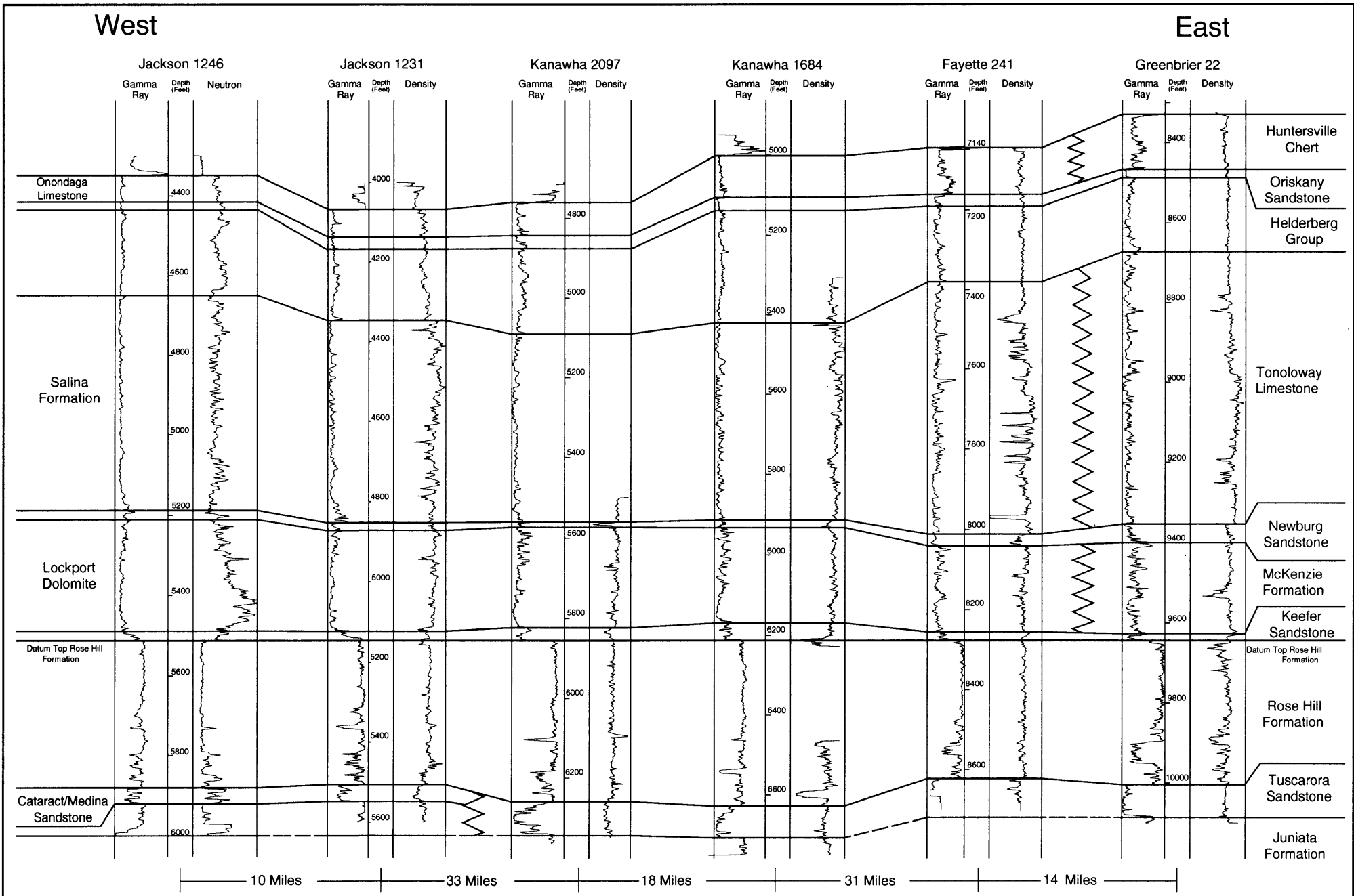
Figure Sts-5. Tuscarora stratigraphic correlations across southern West Virginia, showing the increase in shale content and decrease in thickness of the Tuscarora Sandstone from east to west. The upper part of the Lockport interval also includes the Salina "A" and "B" at the top. Columbia Gas Transmission Corporation No. 8804 Fee (Kanawha 1684) is the designated discovery well for Indian Creek field. The two westernmost wells (Jackson 1246 and Jackson 1231) are outside the play boundary and fall within the Lower Silurian Cataract/Medina Group ("Clinton") sandstone play (see M. McCormac and others, this atlas).
