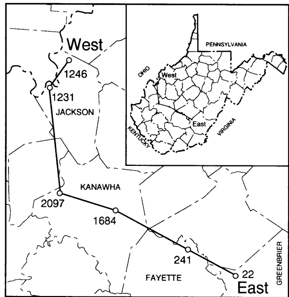
Figure Sts-5. Tuscarora stratigraphic correlations across southern West Virginia, showing the increase in shale content and decrease in thickness of the Tuscarora Sandstone from east to west. The upper part of the Lockport interval also includes the Salina "A" and "B" at the top. Columbia Gas Transmission Corporation No. 8804 Fee (Kanawha 1684) is the designated discovery well for Indian Creek field. The two westernmost wells (Jackson 1246 and Jackson 1231) are outside the play boundary and fall within the Lower Silurian Cataract/Medina Group ("Clinton") sandstone play (see M. McCormac and others, this atlas).
