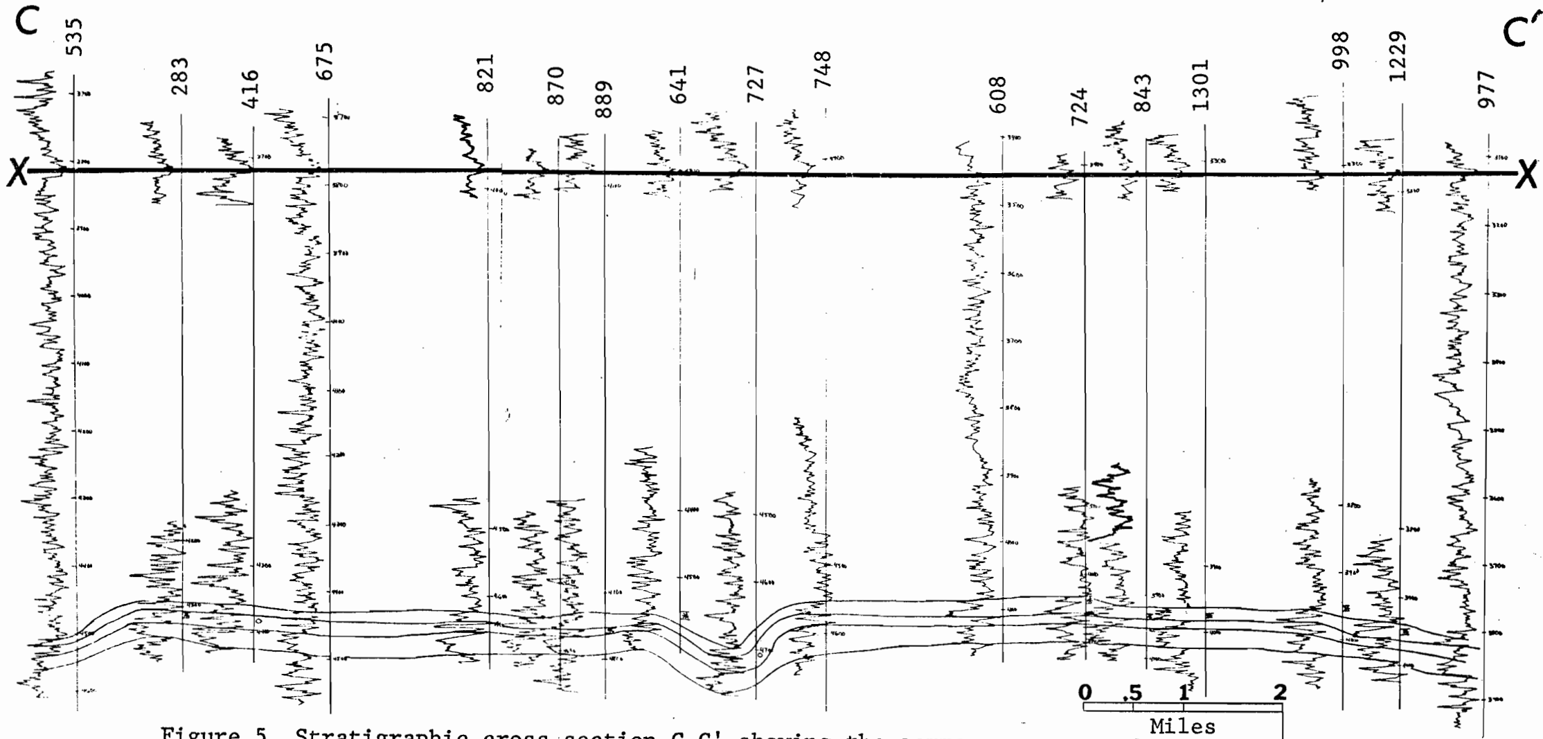
Figure 5. Stratigraphic cross section C-C' showing the gamma-ray log correlation of the three units of the Benson zone based on the radioactive datum (thick line) labelled X. Numbers listed are well permit numbers, * indicates gas production and o indicates a dry hole. Depths on the vertical scale are drilling depths.
