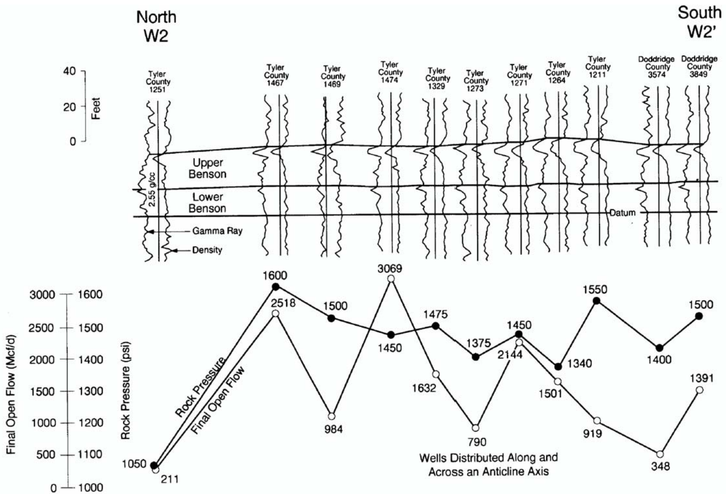
Figure Des-29b. Stratigraphic cross section across the Wilbur field, Doddridge and Tyler counties, West Virginia, showing final open flow and rock pressure.
