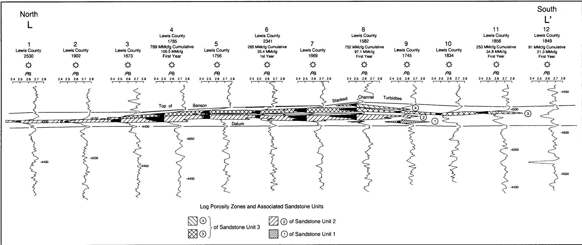
Figure Des-26. Bulk density log stratigraphic cross section across the Weston-Jane Lew field, Lewis County, West Virginia. See Figures Des-22 and Des-24 for location.
