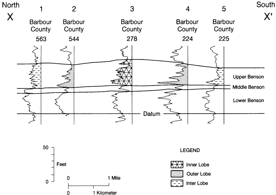
Figure Des-17b. Gamma-ray log cross section X-X' across the inner lobe/channel subfacies trend for the upper Benson reservoir. Note log signatures for the three subfacies of the proximal facies of the slope apron deposits. See Figure Des-17a for location of cross section.
