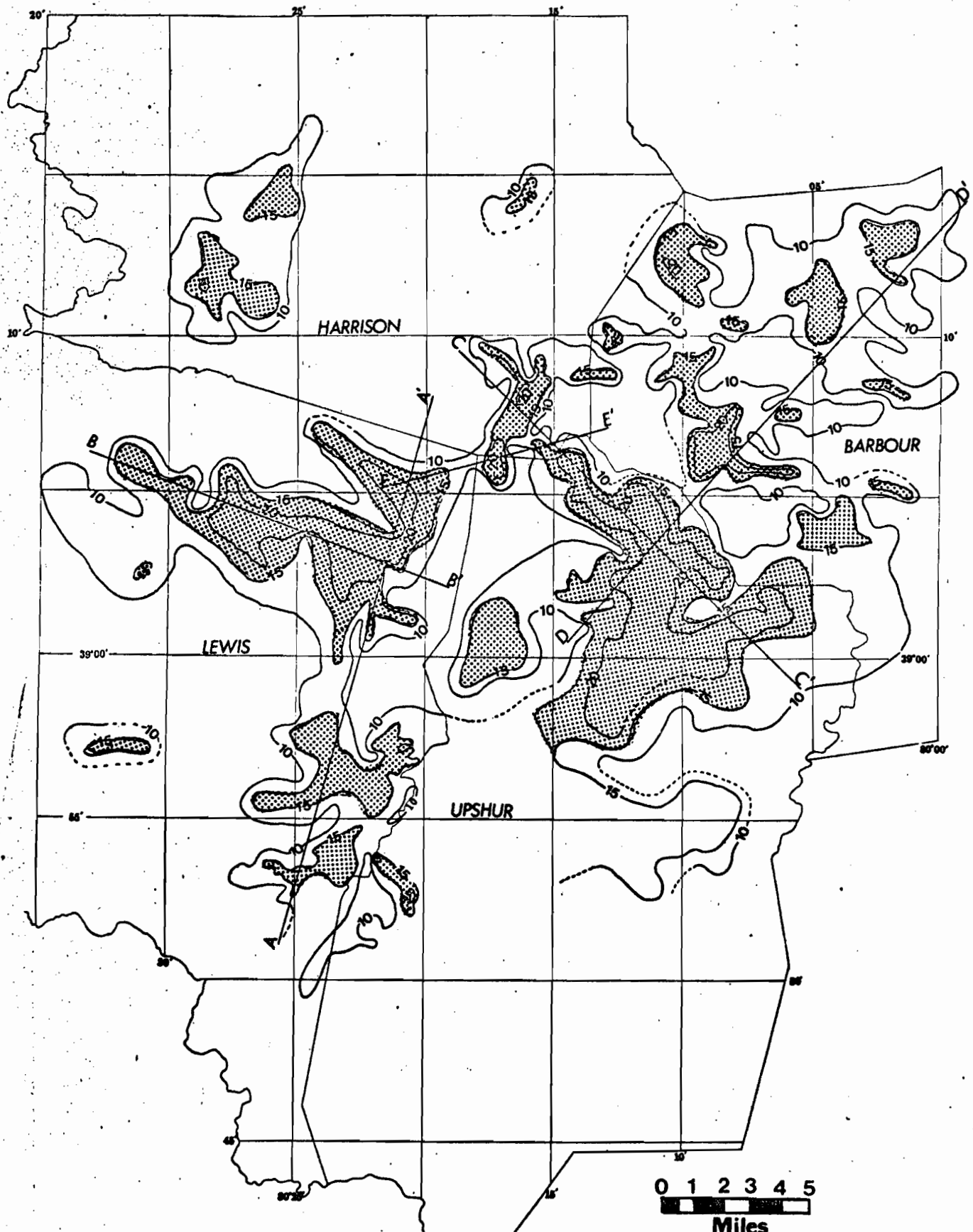
Figure 25. Isolith map of the upper sand in the Benson zone with thickness as interpreted from gamma ray logs. Sand thicknesses of 15 feet and greater are shaded. Contour interval 5 feet. Solid lines indicate cross section locations.
