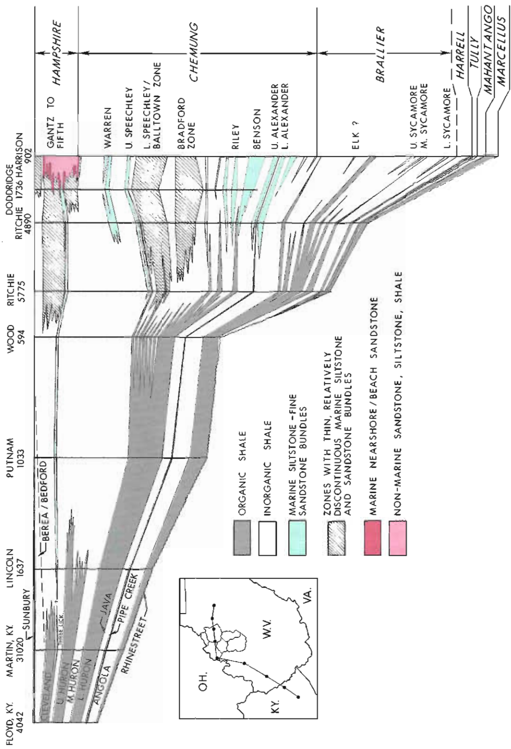
Figure 5. Upper and Middle Devonian fine-grained clastics facies, central West Virginia to eastern Kentucky.
