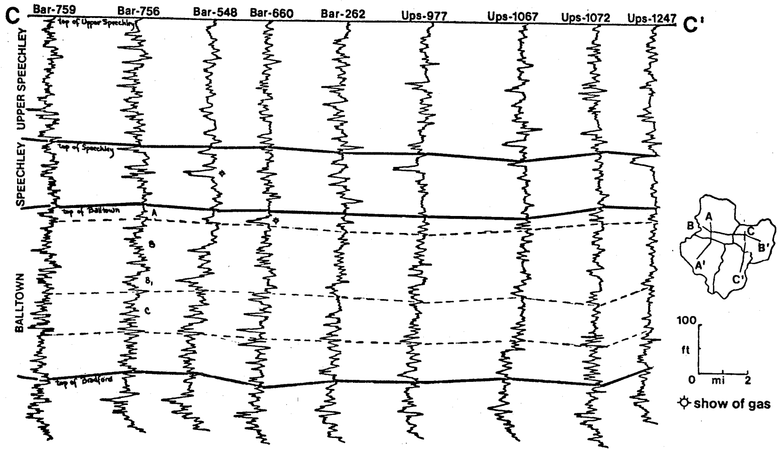
Fig. 6. Transverse (north-south) cross-section across study area. Datum: top of Warren shale.
