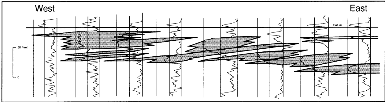
Figure Dbs-31. Gamma-ray log stratigraphic cross section across the Cush Cushion field showing the prograding nature of the productive Kane (B-1) sandstone. Modified from Hussing (1994). See Figure Dbs-2 for location of Cush Cushion field. Well log locations held confidential upon request.
