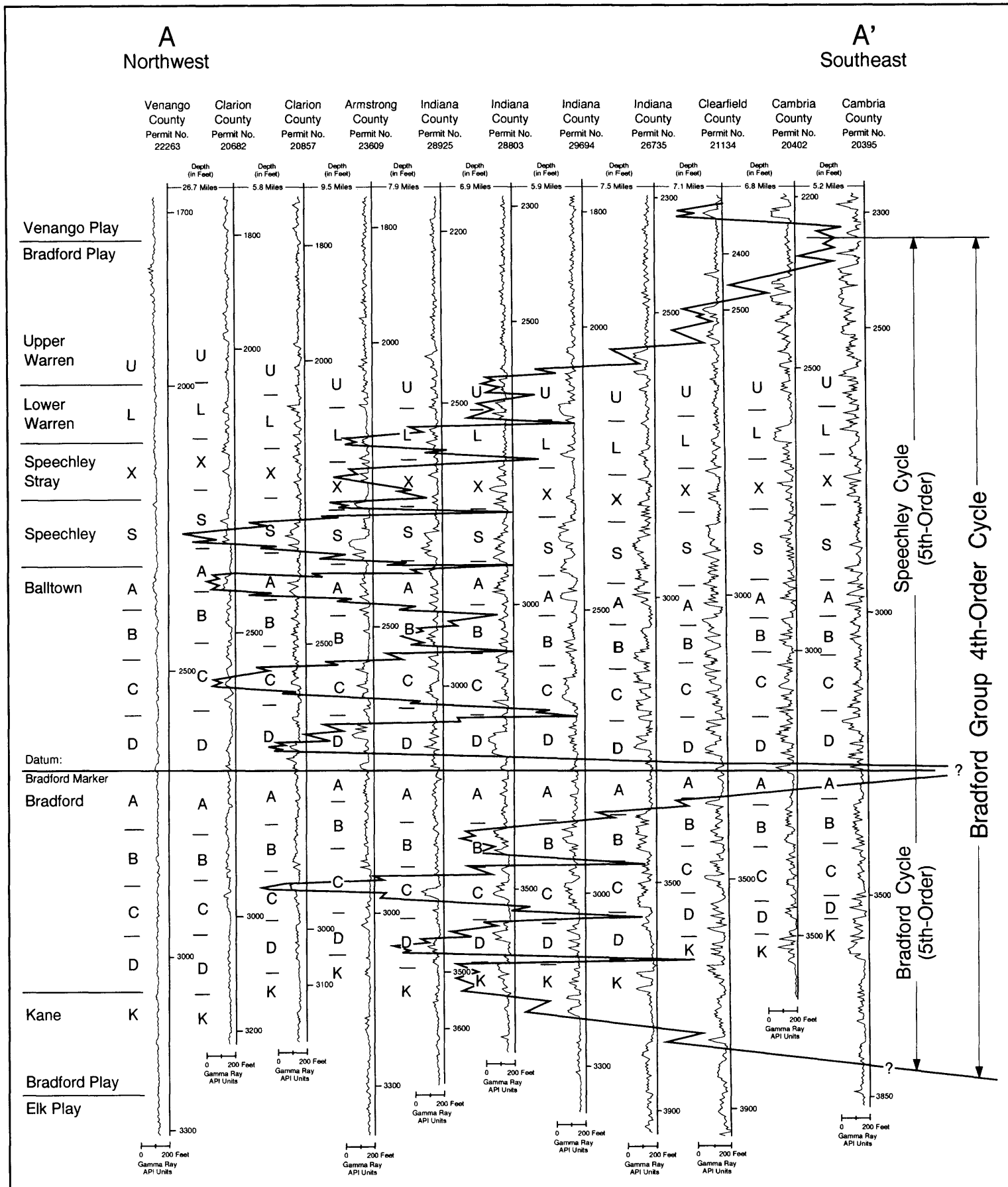
Figure Dbs-8. Stratigraphic cross section A-A' of the Bradford play in Pennsylvania prepared by Flaherty (1994). Based on a network of similar cross sections, Flaherty interpreted two primary transgressive-regressive cycles within the Bradford play, which he named the Bradford cycle (intervals B-1 and B-2) and the Speechley cycle (intervals B-3, B-4, and B-5). Smallest-scale cycles are considered to be sixth order. Figure modified slightly to show atlas intervals. Location of north-south cross section (Figure Dbs-9) is also shown.
