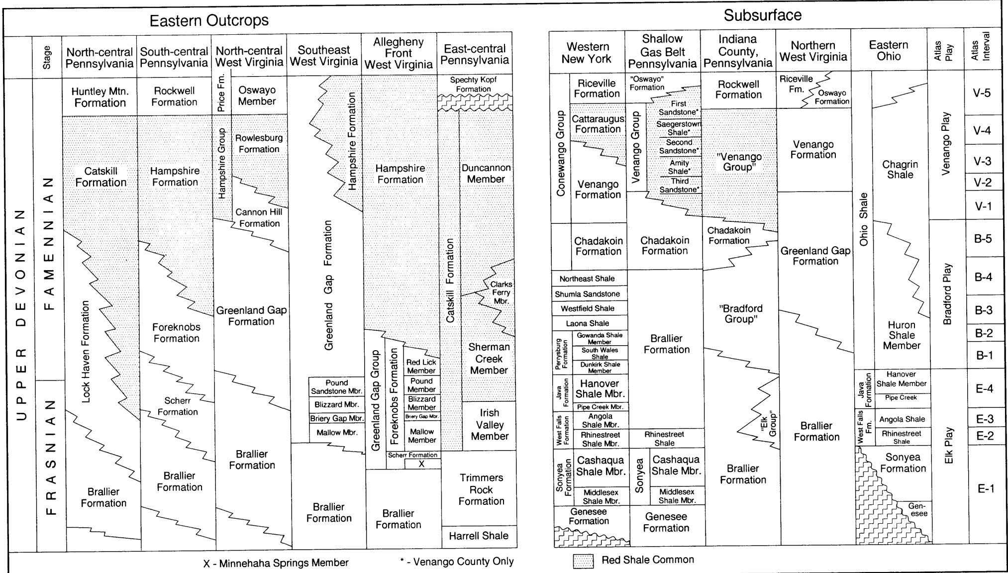
Figure Dbs-5. Regional lithostratigraphy of the Upper Devonian Catskill delta complex. After Boswell and others (1987) and Woodrow and others (1988). The correlation of formations to the stages is approximate and has not been consistently reported in the literature.
