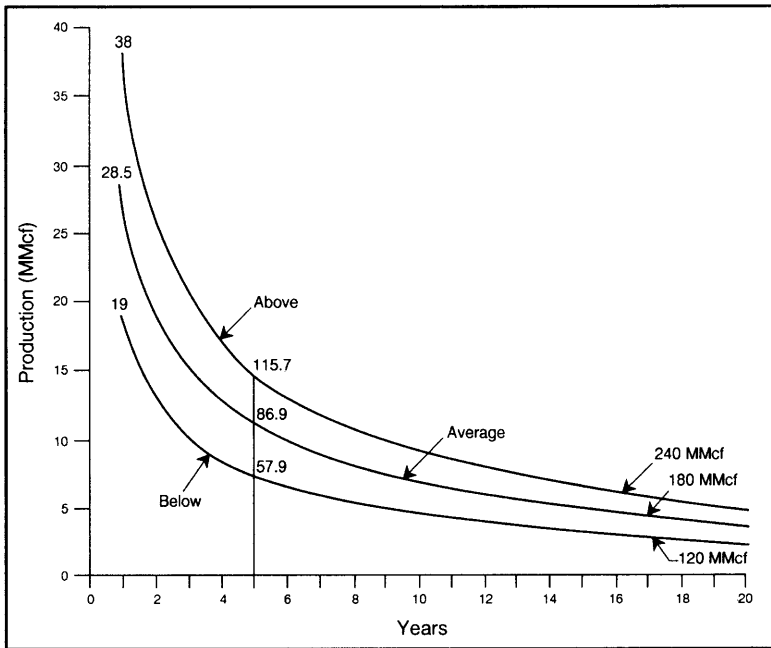
Figure Dbs-19. Typical production decline curve for Bradford wells in Indiana County, Pennsylvania. Profiles for above-average, average, and below-average producing wells are provided. Modified slightly from Harper and others (1996), based on information provided by J. Wigal.
