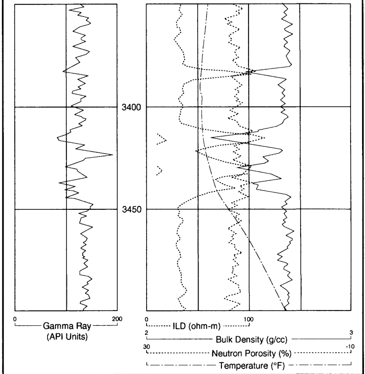
Figure Dbs-28. Type log of porous zone within the B-4 interval in northern Harrison County, West Virginia. Well log name and number held confidential upon request.
