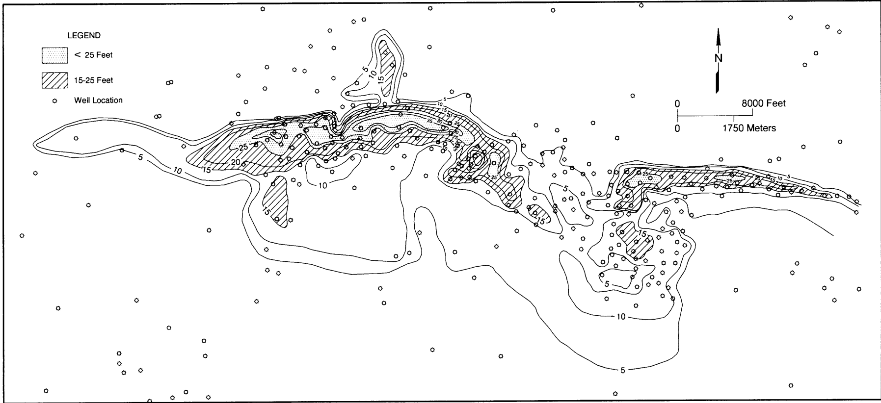
Figure Dbs-30. Sandstone isopach map (greater than 60 percent clean sandstone using the gamma-ray base-line method) of the Kane sandstone (B-1), Cush Cushman field, Clearfield, Indiana, and Cambria counties, Pennsylvania. From Hussing (1994). Contour interval = 5 feet. See Figure Dbs-2 for location.
