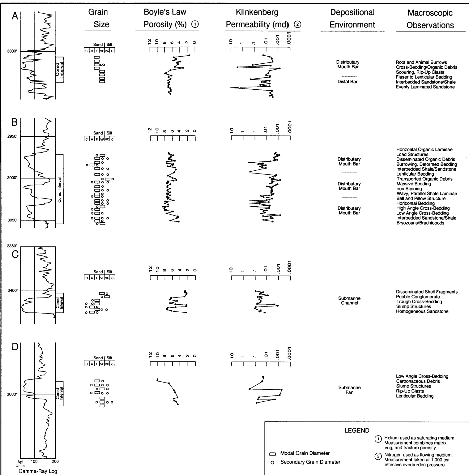
Figures Dbs-16a-d. Core data from the First Bradford (B-2) sandstone from four wells in west-central Pennsylvania; Figure Dbs-16a. No. 1 Good, Lahr, and Kaufman (Indiana County No. 25084). Figure Dbs-16b. No. 1 Beatty (Clearfield County No. 21356). Figure Dbs-16c. No. 3 Stewart (Armstrong County No. 22349). Figure Dbs-16d. No. 1 Shirer (Westmoreland County No. 21640). Modified from Murin (1988). (Boswell and others, 1996-Dbs)
