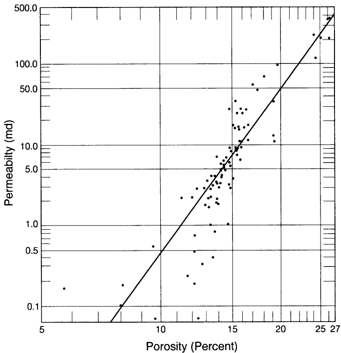
Figure Dbs-12. Relationship of porosity to permeability in three cores of the Bradford Third sandstone reservoir in the Bradford oil field. From Fettke (1938b).
