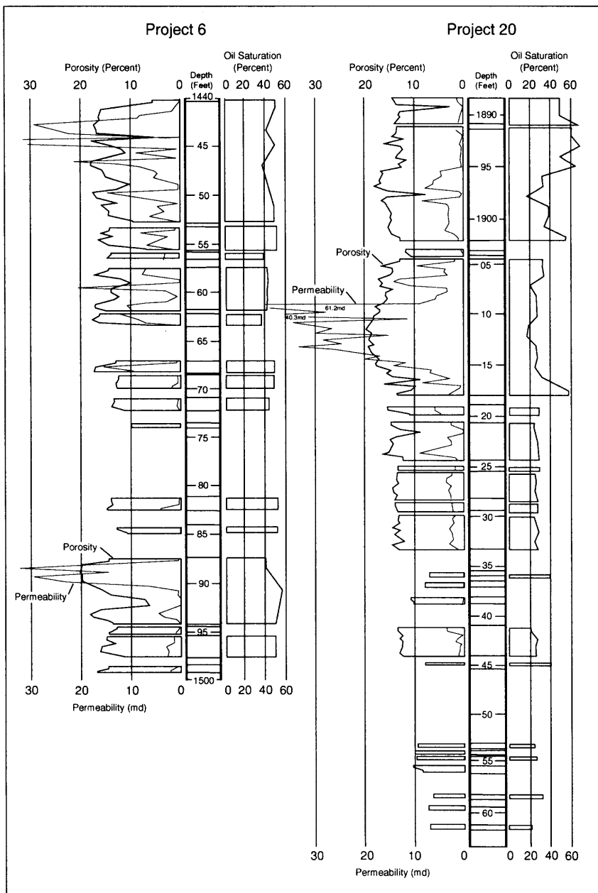
Figure Dbs-11. Graphs of porosity, permeability, and oil saturation of the Bradford Third sandstone (B-1) derived from core analysis of two wells in the Bradford oil field, McKean County, Pennsylvania. From Fettke (1950).
