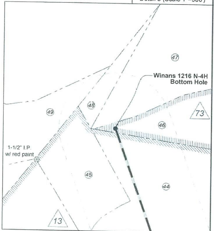
Detail 2 (Scale 1"=500')
