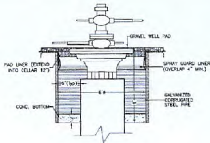
WELL HEAD CELLAR DETAIL
