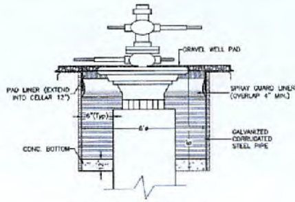
WELL HEAD CELLAR DETAIL N.T.S.
