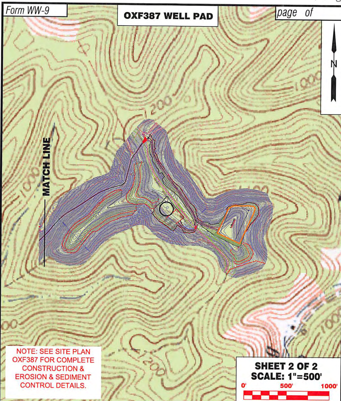
Detail Sketch for Proposed OXF387 Wells
